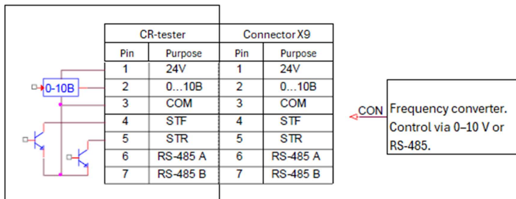
Figure 11. Frequency Converter Connector
