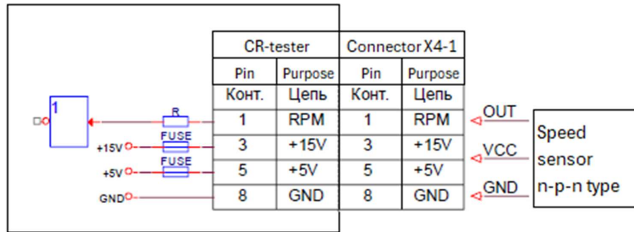
Figure 8. RPM sensor connector
