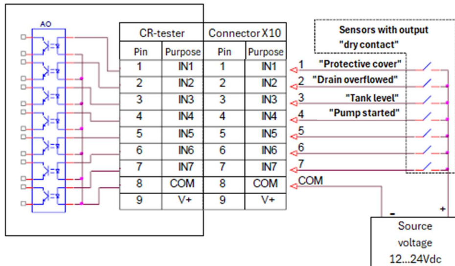
Figure 13. Socket for connecting actuator sensors. Option using external power sensors.
