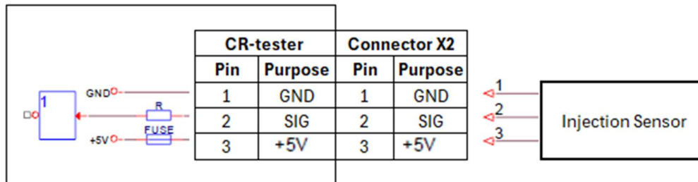
Figure 3. Injection sensor connector
