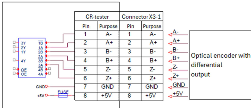
Figure 7. Encoder Connector
