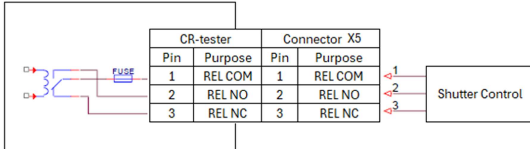
Figure 6. Socket for connecting to a curtain or pump control relay
