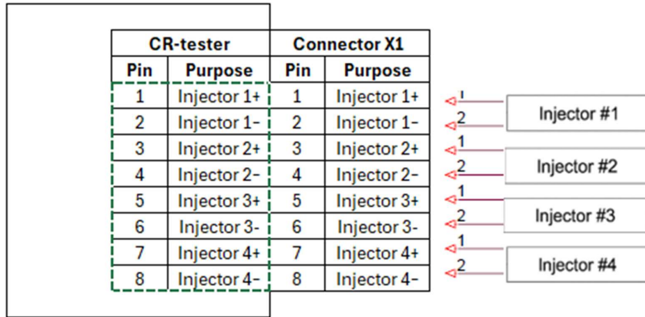
Figure 1. Injector connector (4-injector version)
