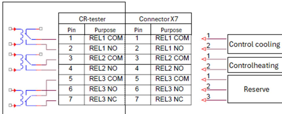
Figure 9. Heater / Cooling Control Connector
