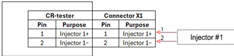
Figure 2. Injector connector (1-injector version)
