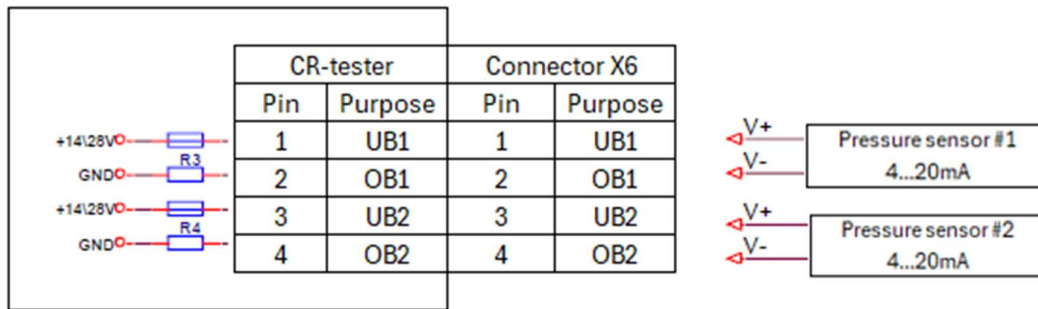
Figure 5. Sensor Connector with 4-20mA Output
