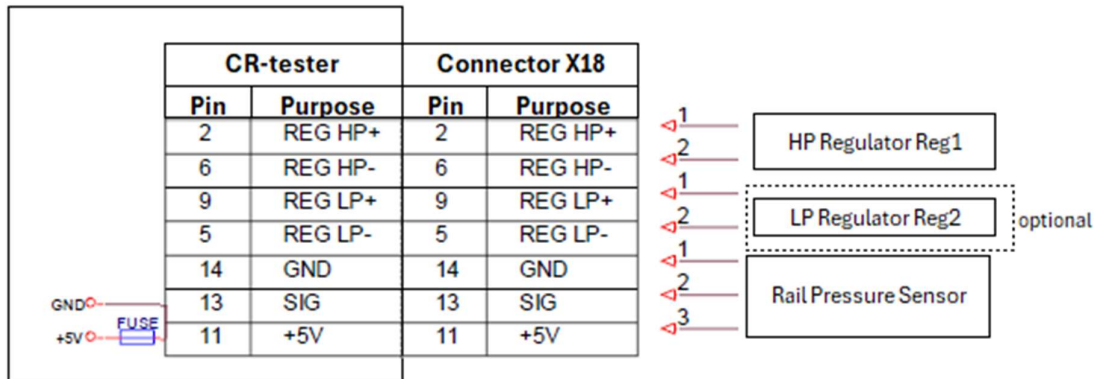
Figure 4. Connector for rail pressure sensor and pressure regulators
