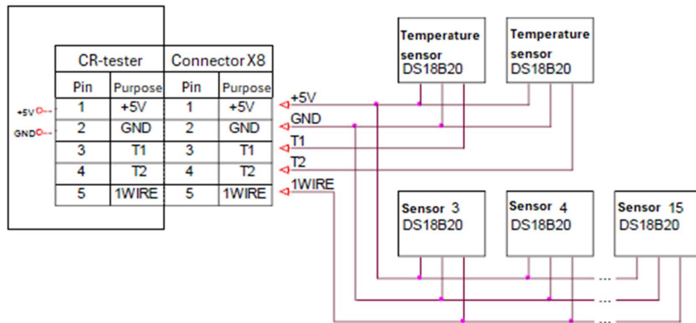
Figure 10. Temperature Sensor Connector
